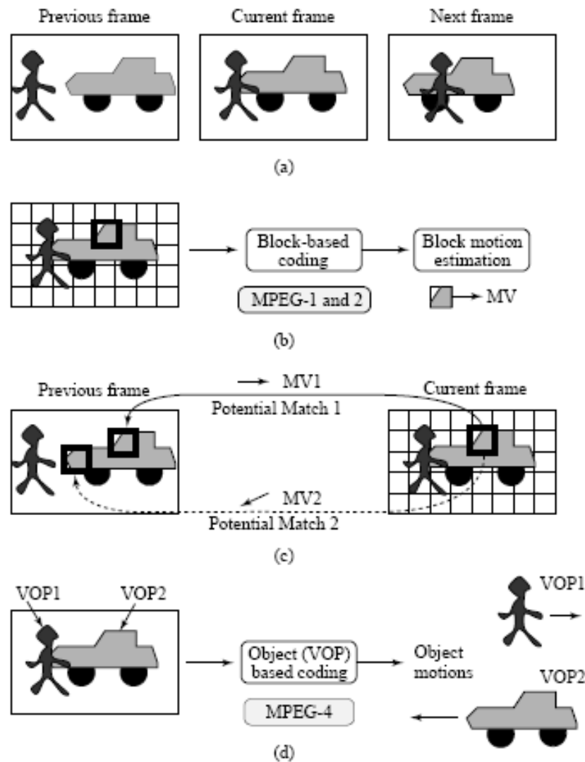
Fig. 12.4: Comparison between Block-based Coding and Object-based Coding.
