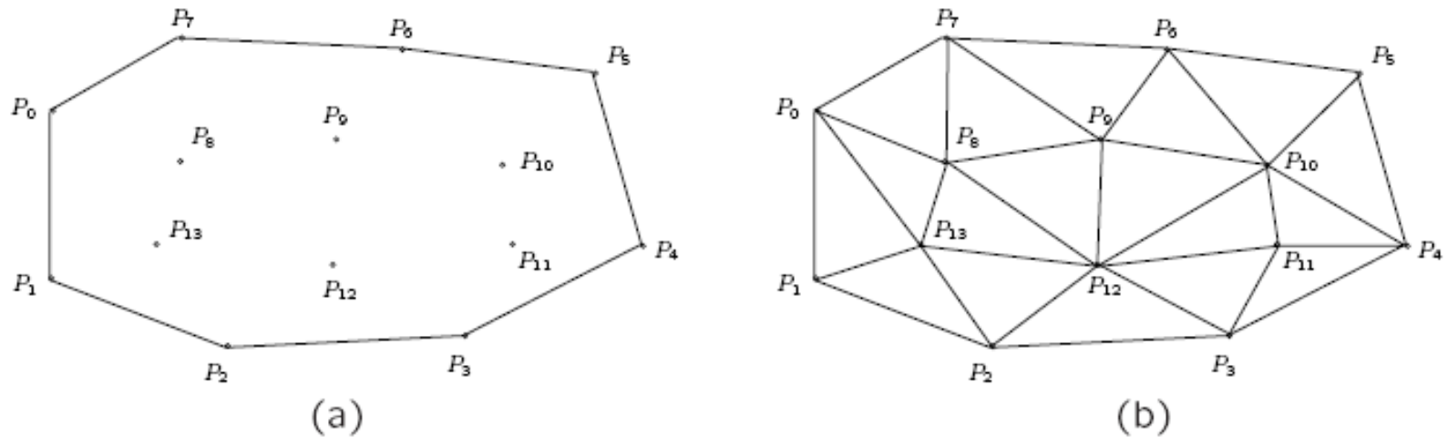
Fig. 12.13: Delaunay Mesh: (a) Boundary nodes ( P_0 to P_7 ) and Interior nodes ( P_8 to P_{13} ). (b) Triangular mesh obtained by Constrained Delaunay Triangulation.
