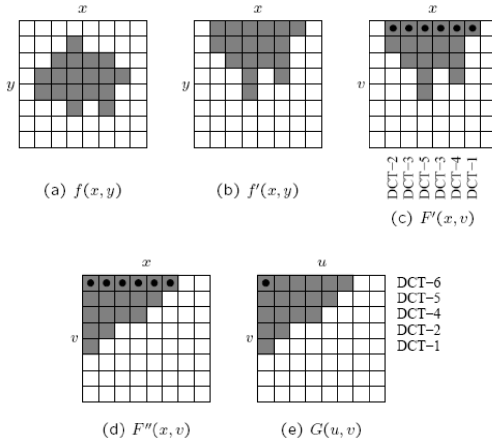
Fig. 12.8: Texture Coding for Boundary MBs Using the Shape Adaptive DCT (SA-DCT).
